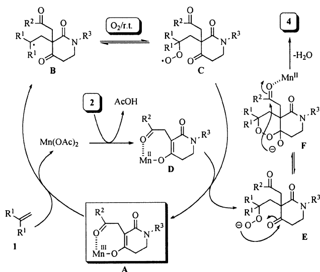
Scheme 9. Proposed mechanism for the Mn III -catalyzed aerobic oxidation of 3-(2-oxoethyl)piperidine-2,4-diones 2 in the presence of alkenes 1 .
