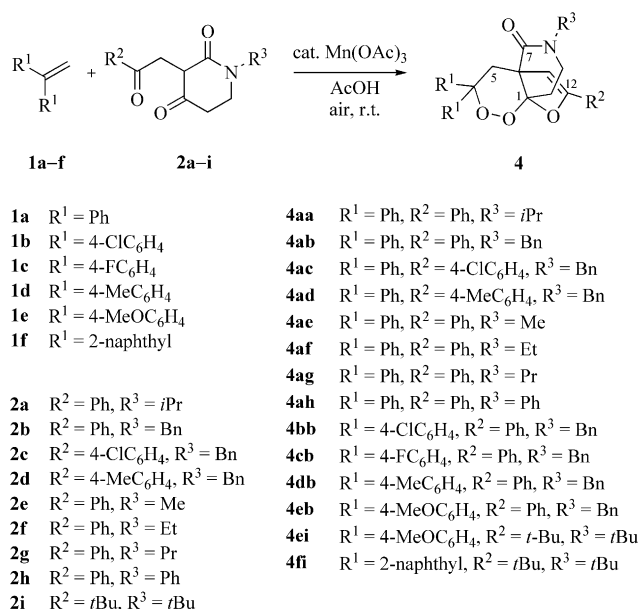
Scheme 2. Mn III -mediated aerobic oxidation of a combination of 1,1-diarylethenes 1 and 3-(2-oxoethyl)piperidine-2,4-diones 2 at room temperature.
