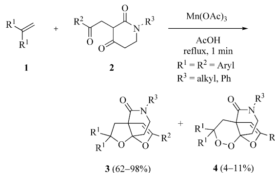
Scheme 1. Oxidation of 2-oxoethyl-substituted piperidine-2,4-diones 2 with manganese(III) acetate in the presence of 1,1-diarylethenes 1 at reflux temperature.
