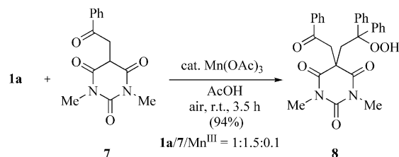
Scheme 4. Mn III -catalyzed aerobic oxidation of a combination of 1,1-diphenylethene ( 1a ) and 5-(2-oxoethyl)barbituric acid 7 at room temperature.
