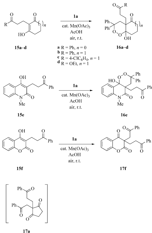
Scheme 7. Similar aerobic oxidation with 3-oxopropyl-substituted cyclic 1,3-diones 15a–f .
