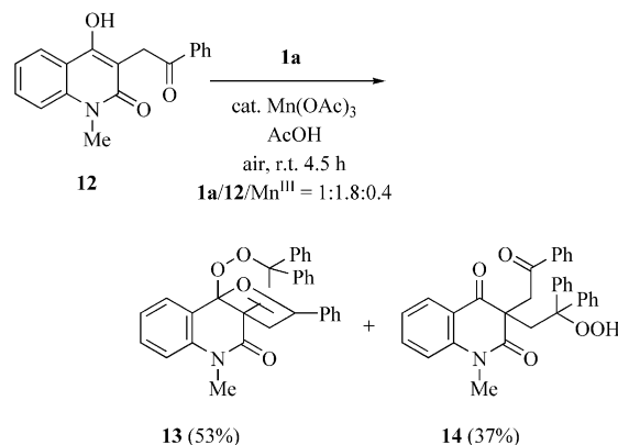
Scheme 6. Mn III -catalyzed aerobic oxidation of 4-hydroxy-3-(2-oxoethyl)-1 H -quinolin-2-one ( 12 ) at room temperature.
