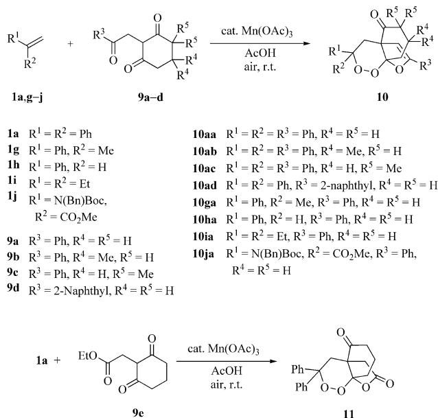
Scheme 5. Mn III -catalyzed aerobic oxidation of a combination of alkenes 1 and 2-(2-oxoethyl)cyclohexane-1,3-diones 9 at room temperature.
