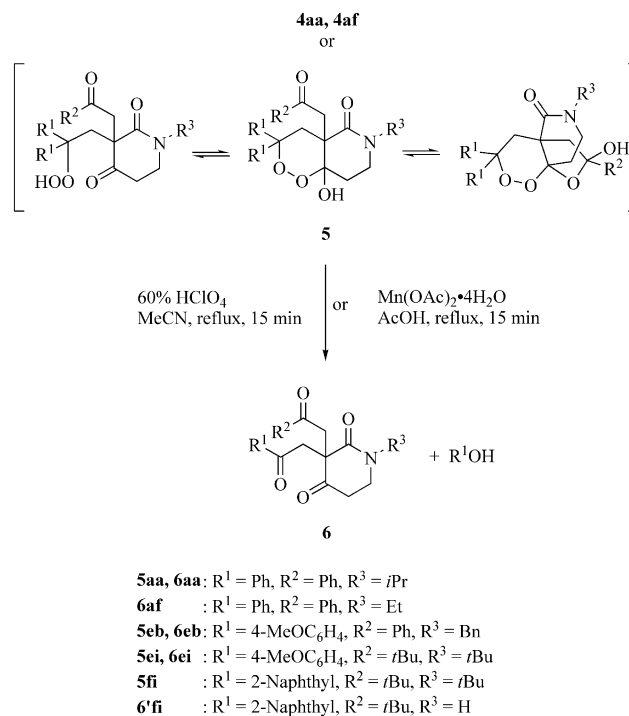
Scheme 3. Acid-catalyzed decomposition of azatrioxapropellanes 4aa, 4af or the propellane precursors 5 .
